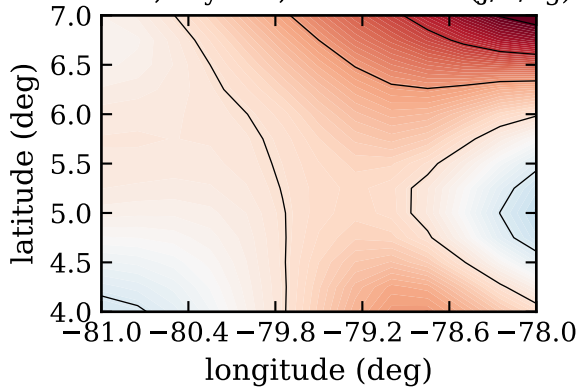
RF09a, day 237, instab index (J/K/kg)
