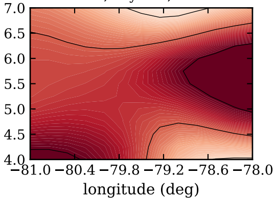
RF09a, day 237, satfrac
