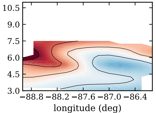
RF11, day 247, satfrac
