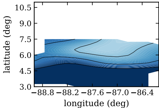
RF11, day 247, instab index (J/K/kg)
