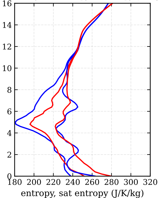
RF11, day 247 - entropy, sat entropy (J/K/kg)
