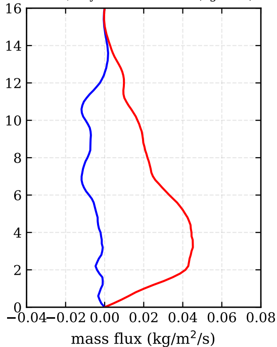
RF11, day 247 - mass flux (kg/m 2 /s)
