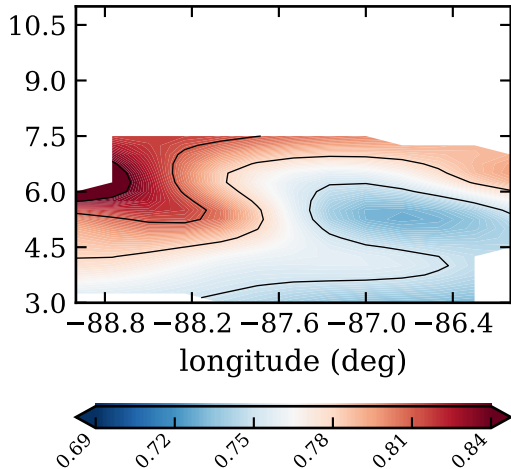
RF11, day 247, satfrac
