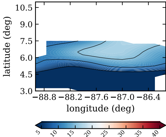
RF11, day 247, instab index (J/K/kg)
