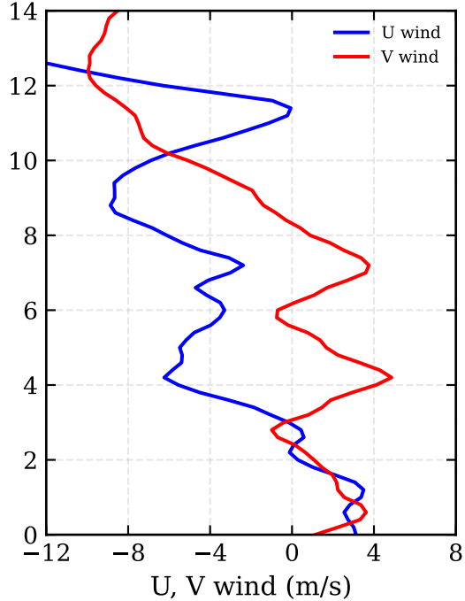
RF11: 3DVAR (-89.0, 6.0) - U wind / V wind
