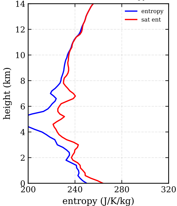
RF11: 3DVAR (-89.0, 6.0) - entropy / sat ent
