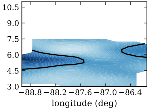
RF11, day 247, srcent ( \text{W}/\text{m}^2 )
