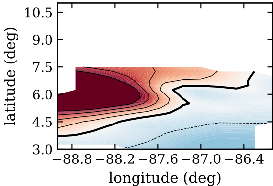
RF11, day 247, srcmr, ( \text{W}/\text{m}^2 )
