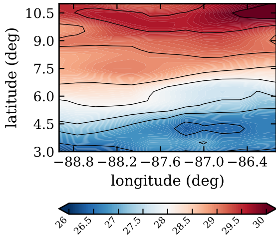
RF11, day 247, SST (C)
