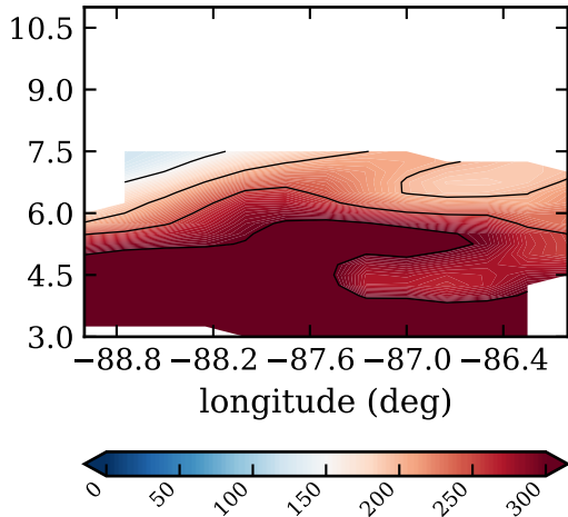
RF11, day 247, eflux (W/m 2 )
