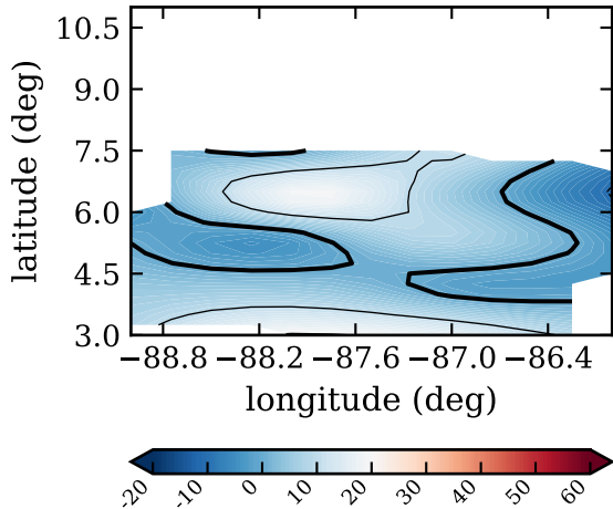
RF11, day 247, dcin, (J/K/kg)
