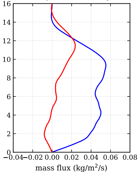
RF13c, day 260 - mass flux (kg/m 2 /s)
