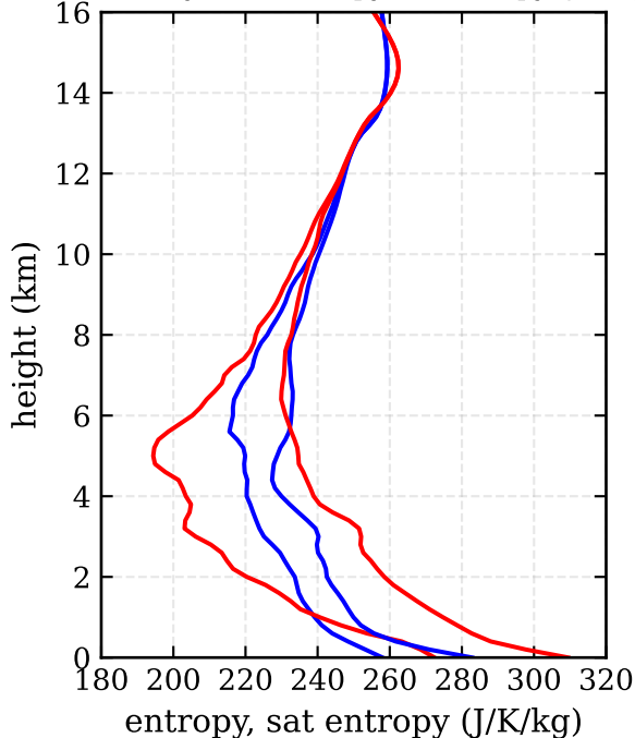
RF13c, day 260 - entropy, sat entropy (J/K/kg)
