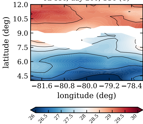
RF13c, day 260, SST (C)
