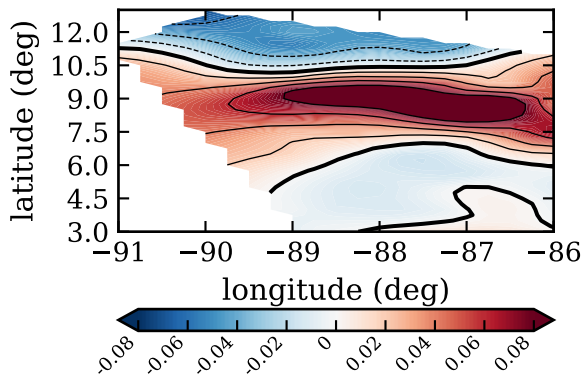
RF14, day 264, mfluxlo (kg/m 2 /s)
