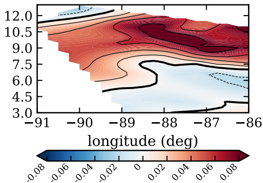
RF14, day 264, mfluxhi (kg/m 2 /s)
