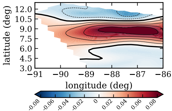
RF14, day 264, mfluxvl (kg/m 2 /s)
