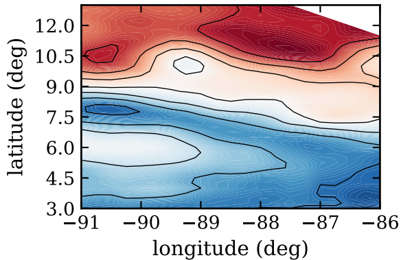
RF14, day 264, SST (C)
