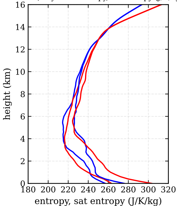
RF15c, day 265 - entropy, sat entropy (J/K/kg)
