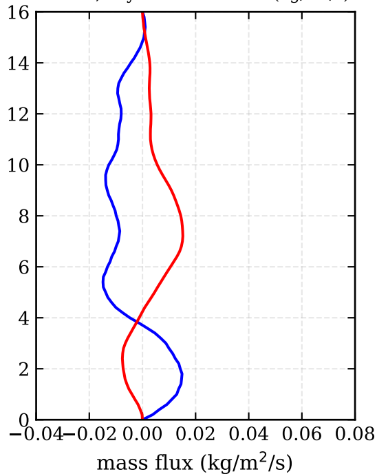
RF15c, day 265 - mass flux (kg/m 2 /s)
