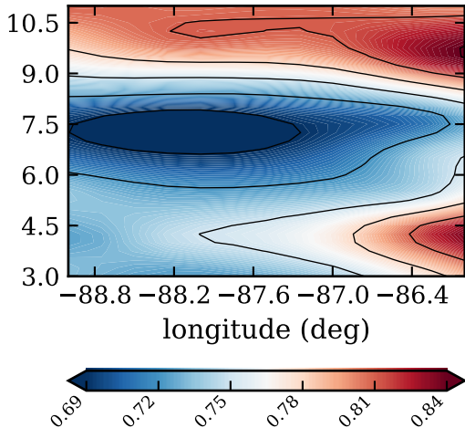
RF16, day 267, satfrac
