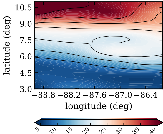
RF16, day 267, instab index (J/K/kg)
