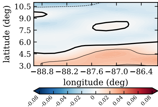
RF16, day 267, mfluxvl (kg/m 2 /s)
