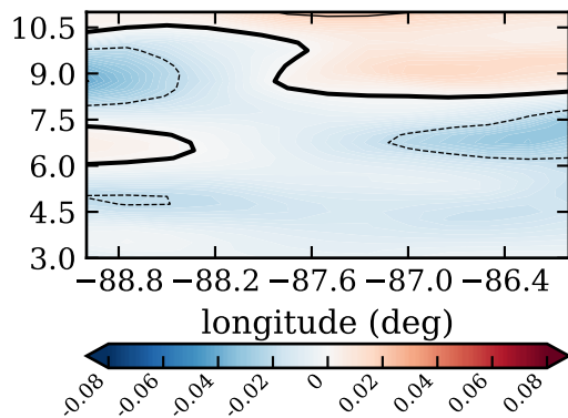
RF16, day 267, mfluxhi (kg/m 2 /s)
