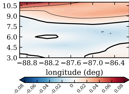
RF16, day 267, mfluxdif (kg/m 2 /s)
