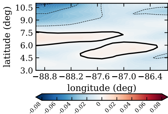
RF16, day 267, mfluxlo (kg/m 2 /s)
