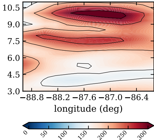
RF16, day 267, eflux (W/m 2 )
