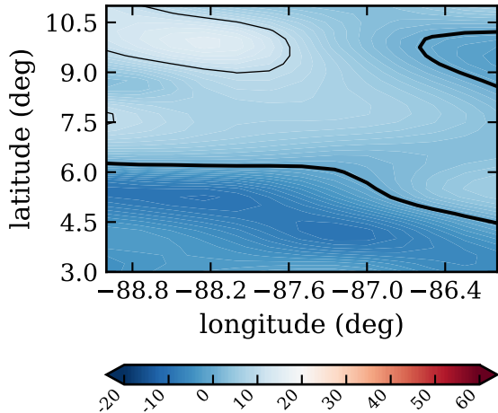
RF16, day 267, dcin, (J/K/kg)
