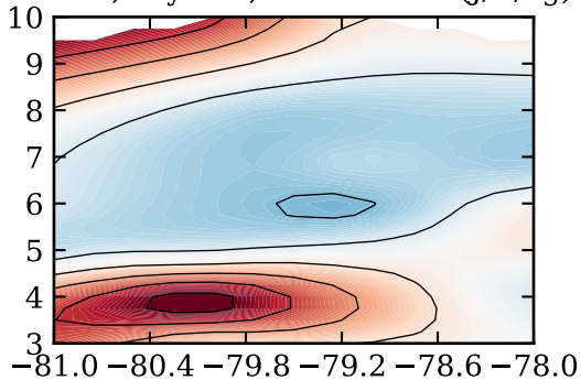
RF17c, day 268, instab index (J/K/kg)
