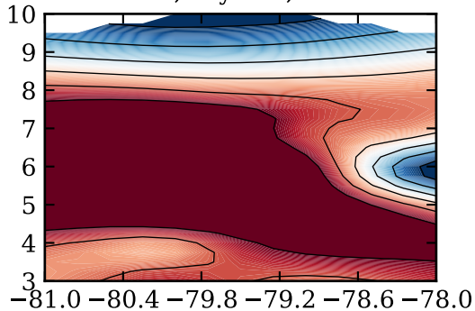
RF17c, day 268, satfrac
