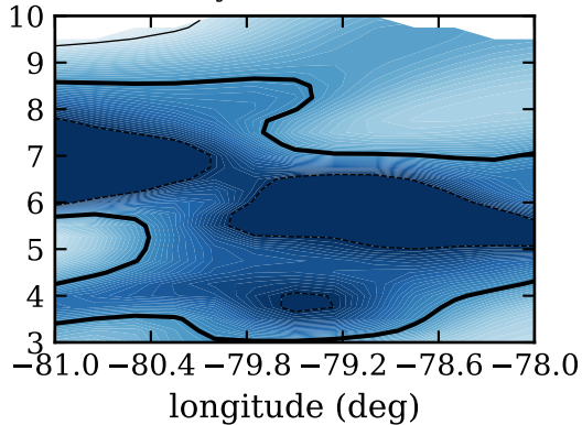
RF17c, day 268, srcent ( \text{W/m}^2 )
