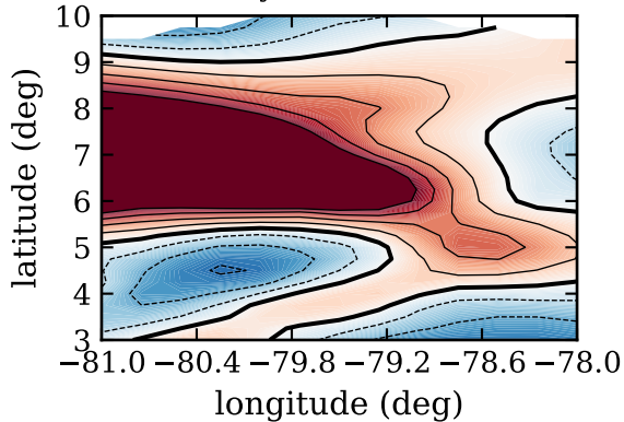
RF17c, day 268, srcmr, ( \text{W/m}^2 )
