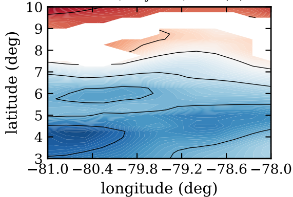
RF17c, day 268, SST (C)
