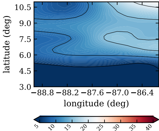
RF18, day 270, instab index (J/K/kg)
