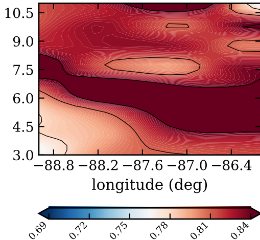
RF18, day 270, satfrac
