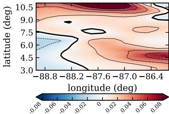
RF18, day 270, mfluxlo (kg/m 2 /s)
