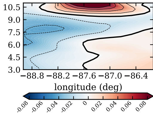
RF18, day 270, mfluxhi (kg/m 2 /s)
