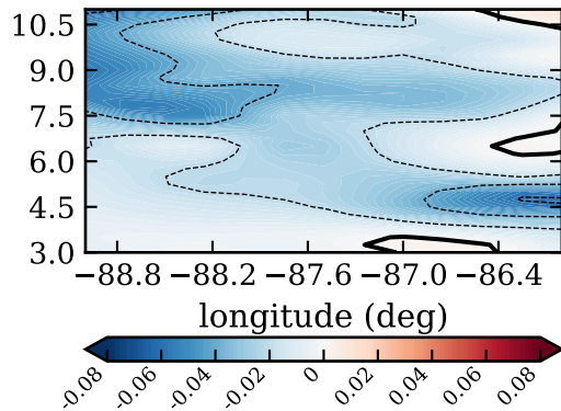
RF18, day 270, mfluxdif (kg/m 2 /s)
