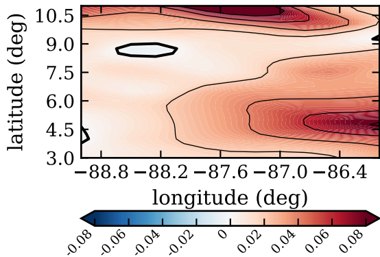
RF18, day 270, mfluxvl (kg/m 2 /s)
