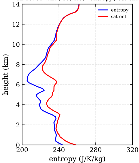
RF18: 3DVAR (-86, 4.8) - entropy / sat ent
