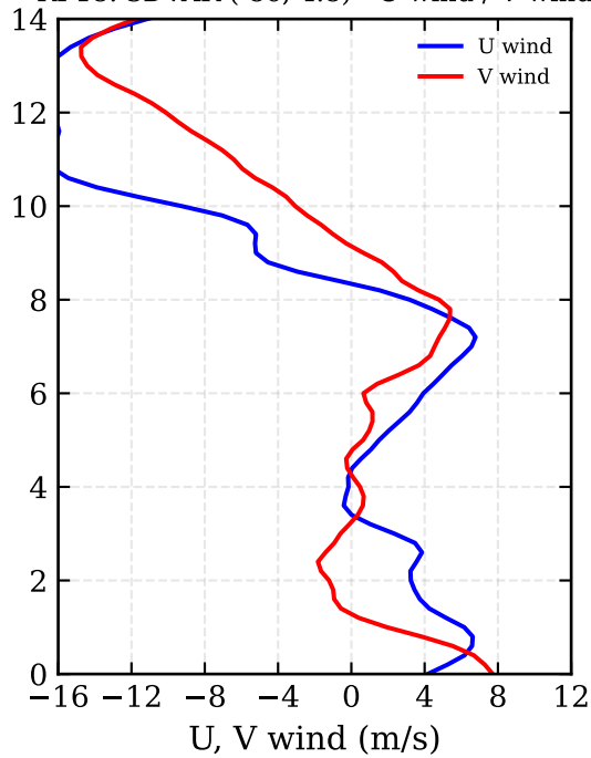
RF18: 3DVAR (-86, 4.8) - U wind / V wind
