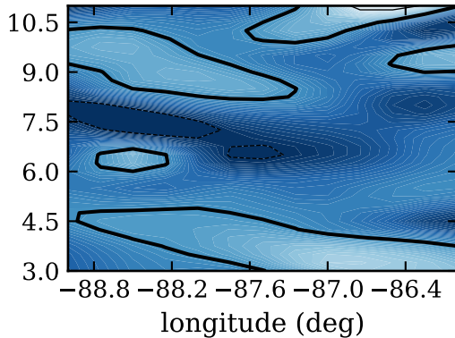
RF18, day 270, srcent ( \text{W/m}^2 )
