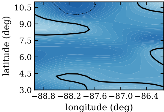
RF18, day 270, dcin, (J/K/kg)
