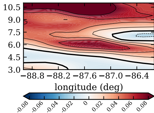
RF19, day 271, mfluxhi ( \text{kg}/\text{m}^2/\text{s} )
