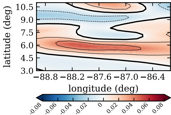
RF19, day 271, mfluxvl ( \text{kg}/\text{m}^2/\text{s} )
