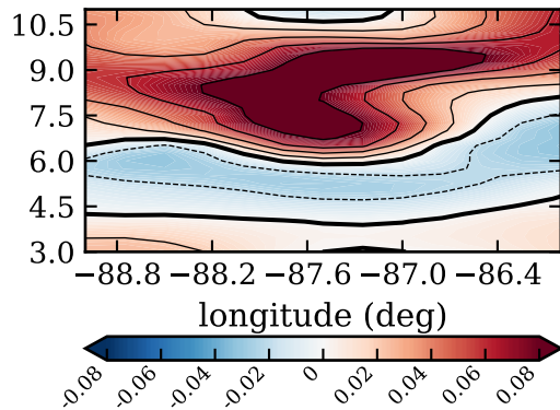
RF19, day 271, mfluxdif ( \text{kg}/\text{m}^2/\text{s} )
