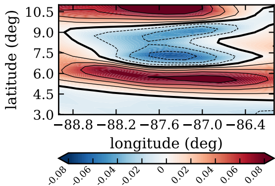
RF19, day 271, mfluxlo ( \text{kg}/\text{m}^2/\text{s} )
