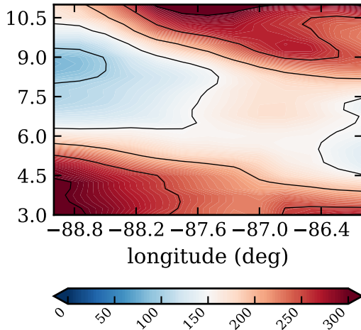
RF19, day 271, eflux (W/m 2 )
