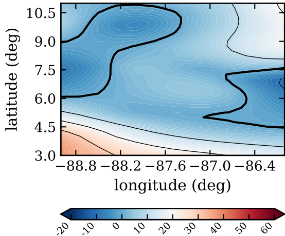
RF19, day 271, dcin, (J/K/kg)
