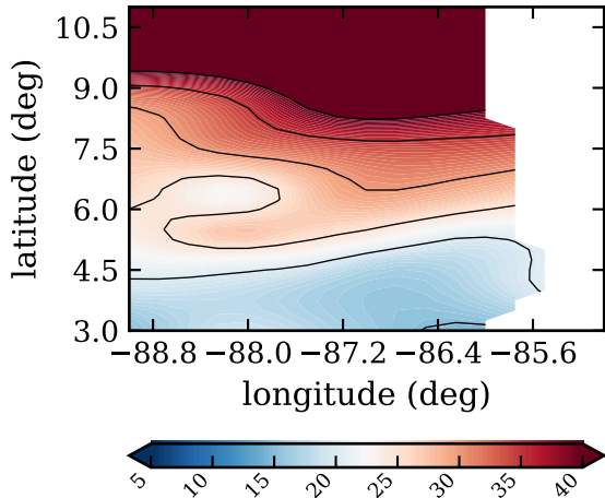
RF20, day 273, instab index (J/K/kg)
