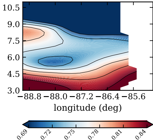
RF20, day 273, satfrac
