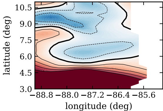
RF20, day 273, srcmr, ( \text{W/m}^2 )
