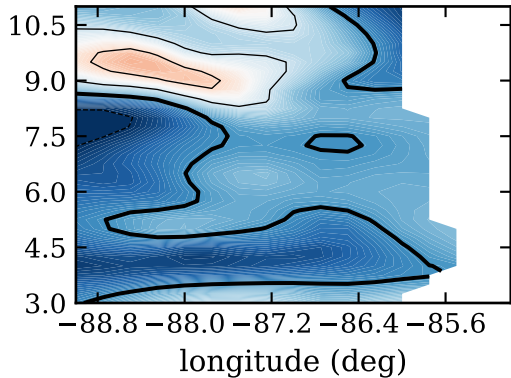
RF20, day 273, srcent ( \text{W/m}^2 )
