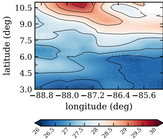
RF20, day 273, SST (C)
