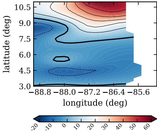
RF20, day 273, dcin, (J/K/kg)
