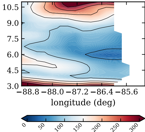
RF20, day 273, eflux (W/m 2 )
