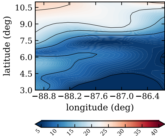
RF21, day 274, instab index (J/K/kg)
