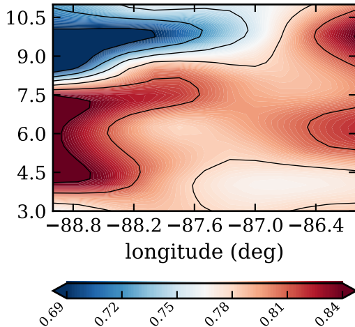
RF21, day 274, satfrac
