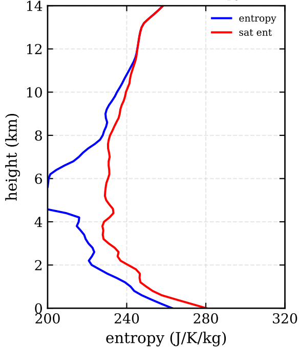
RF21: 3DVAR (-87.7, 8) - entropy / sat ent
