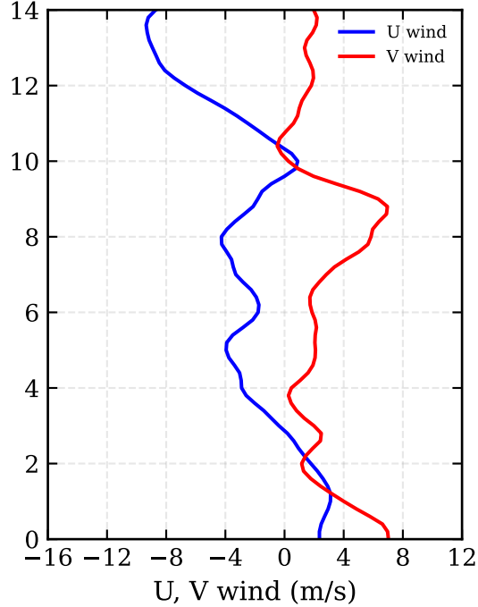
RF21: 3DVAR (-87.7, 8) - U wind / V wind
