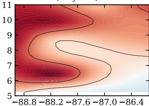
RF22, day 275, satfrac
