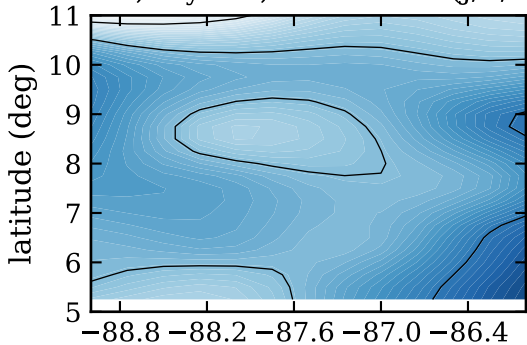
RF22, day 275, instab index (J/K/kg)
