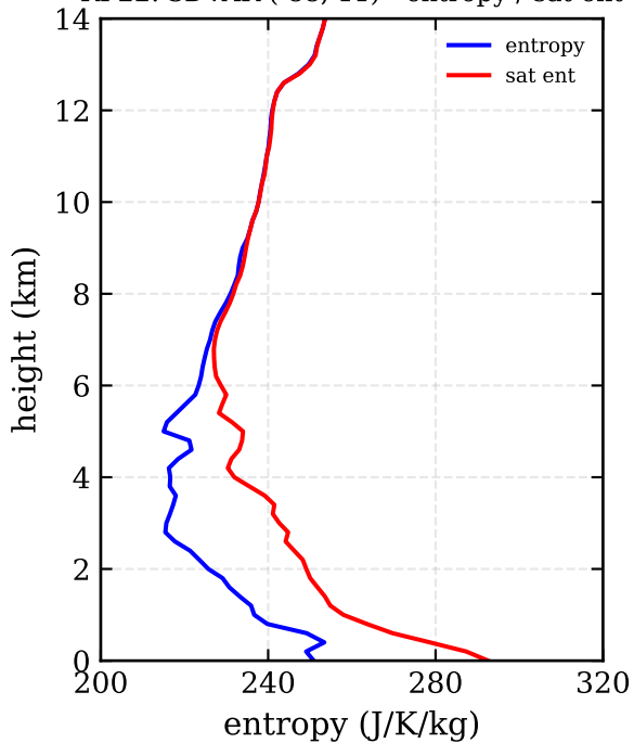
RF22: 3DVAR (-88, 11) - entropy / sat ent
