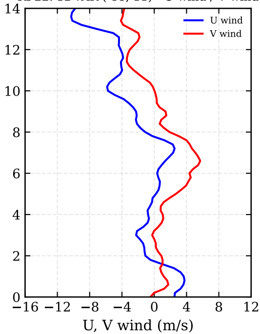
RF22: 3DVAR (-88, 11) - U wind / V wind
