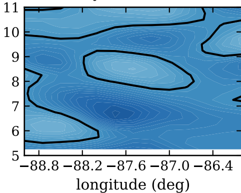
RF22, day 275, srcent ( \text{W/m}^2 )
