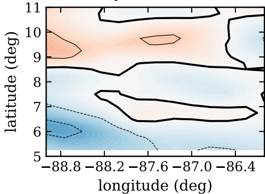
RF22, day 275, srcmr, ( \text{W/m}^2 )
