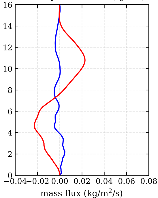
RF01, day 219 - mass flux (kg/m 2 /s)
