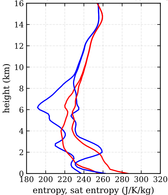
RF01, day 219 - entropy, sat entropy (J/K/kg)
