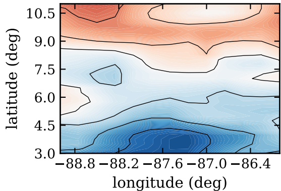
RF01, day 219, SST (C)
