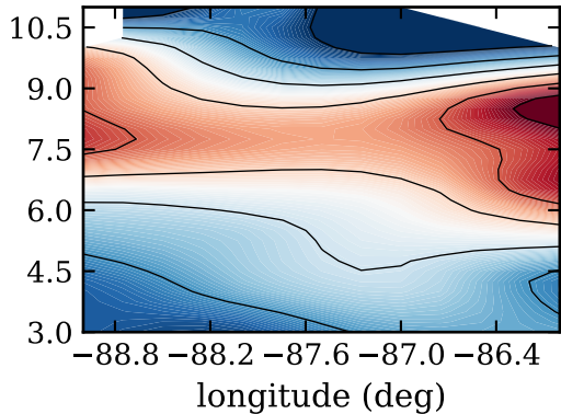
RF03, day 224, satfrac
