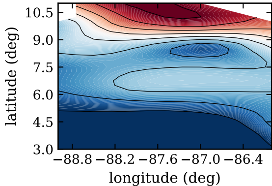
RF03, day 224, instab index (J/K/kg)
