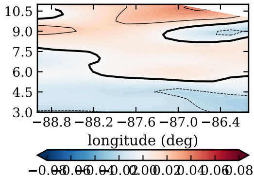
RF03, day 224, mfluxhi (kg/m 2 /s)
