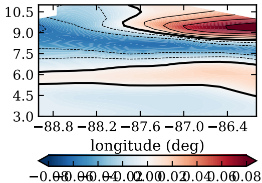
RF03, day 224, mfluxdif (kg/m 2 /s)
