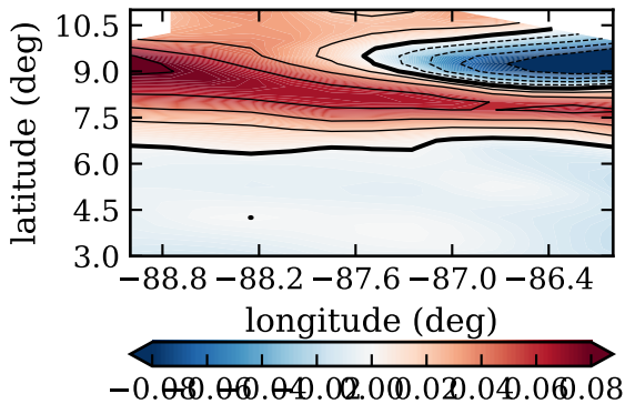
RF03, day 224, mfluxlo (kg/m 2 /s)
