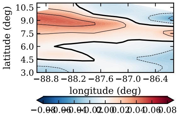
RF03, day 224, mfluxvl (kg/m 2 /s)
