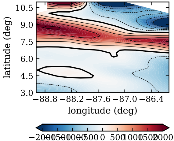
RF03, day 224, srcmr, ( \text{W}/\text{m}^2 )
