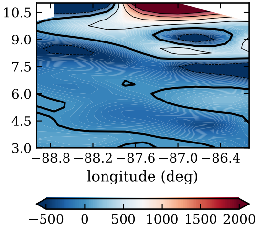
RF03, day 224, srcent ( \text{W}/\text{m}^2 )
