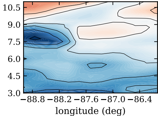
RF03, day 224, SST (C)
