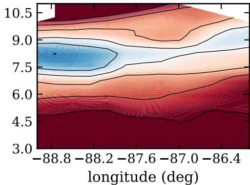
RF03, day 224, eflux (W/m 2 )
