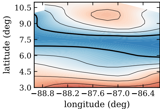
RF03, day 224, dcin, (J/K/kg)
