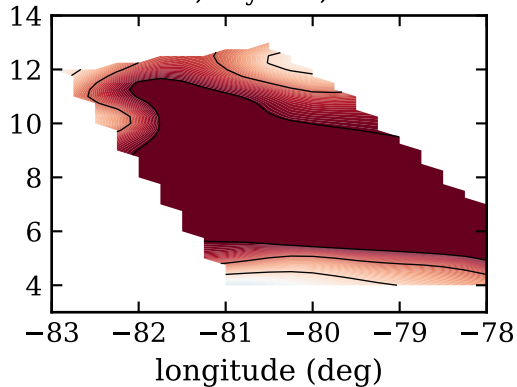
RF04c, day 228, satfrac
