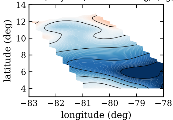
RF04c, day 228, instab index (J/K/kg)
