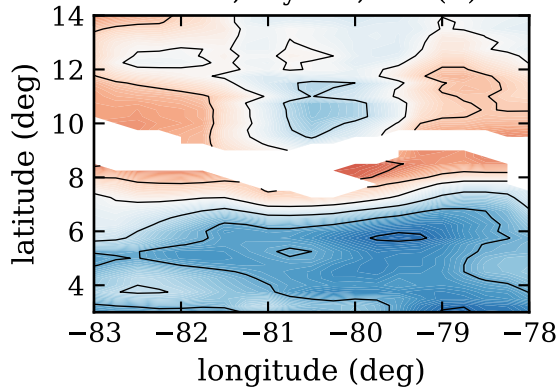
RF04c, day 228, SST (C)
