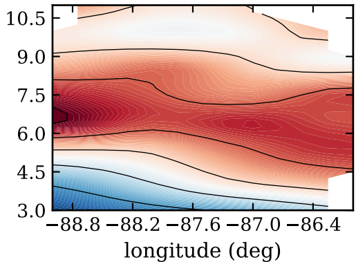
RF05, day 229, satfrac
