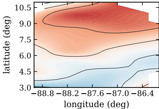
RF05, day 229, instab index (J/K/kg)
