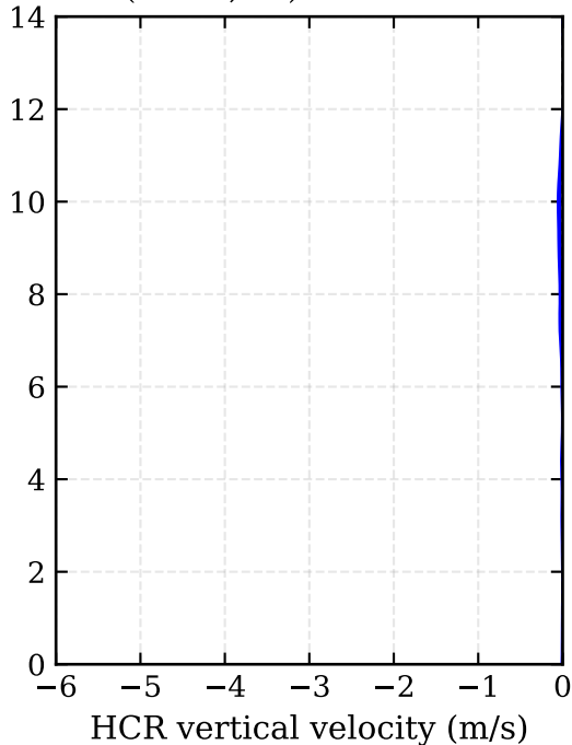
RF05: 3DVAR (-89:-86, 7:8) - HCR vertical velocity (m/s)
