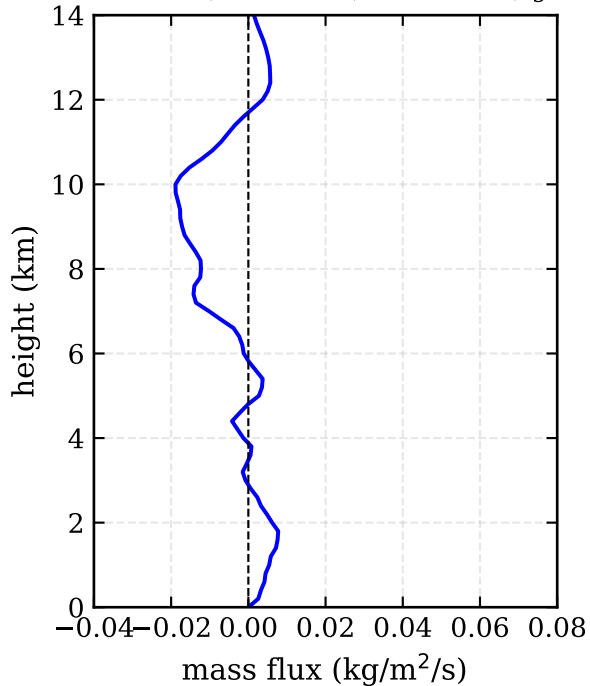
RF05: 3DVAR (-89:-86, 7:8) - mass flux ( \text{kg/m}^2/\text{s} )
