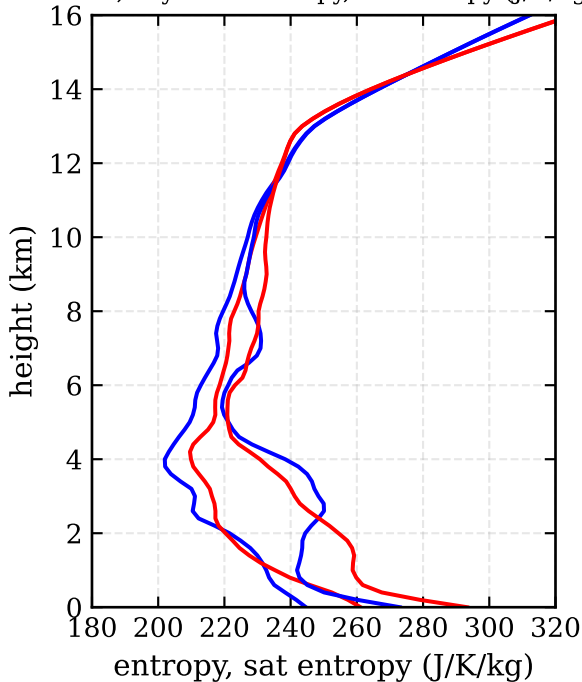
RF05, day 229 - entropy, sat entropy (J/K/kg)
