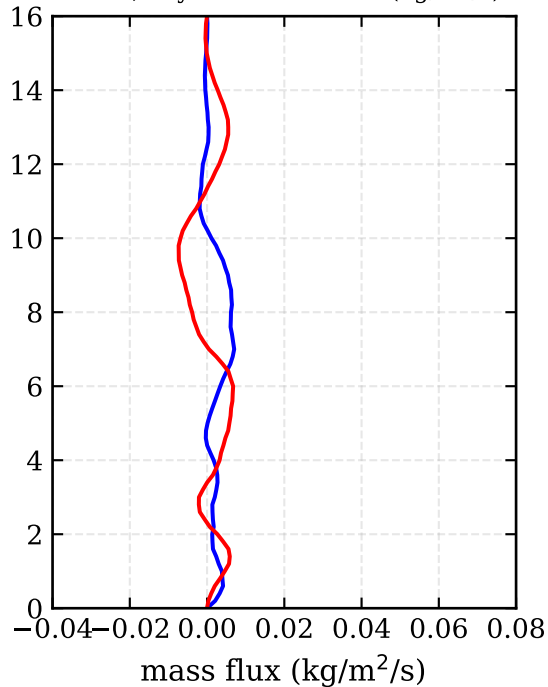
RF05, day 229 - mass flux (kg/m 2 /s)
