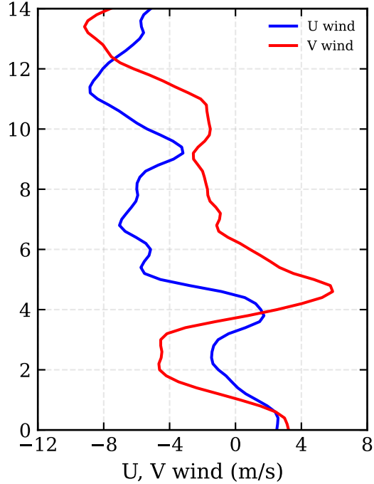
RF05: 3DVAR (-89:-86, 7:8) - U wind / V wind
