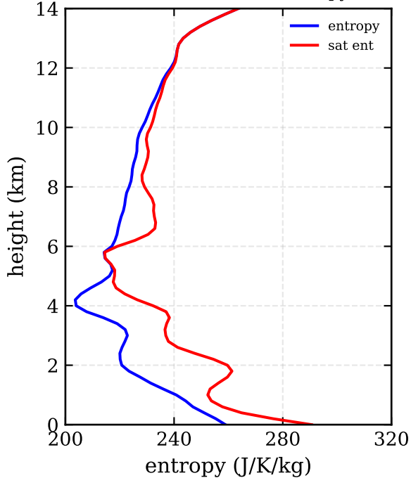
RF05: 3DVAR (-89:-86, 7:8) - entropy / sat ent
