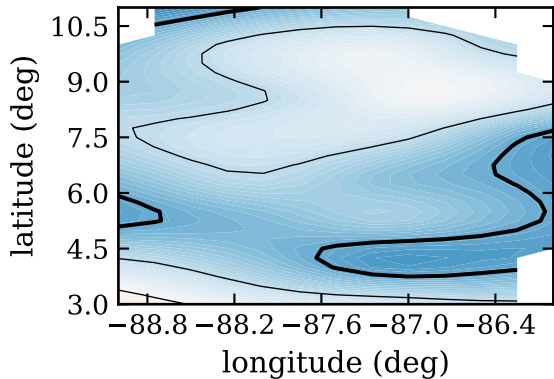
RF05, day 229, dcin, (J/K/kg)
