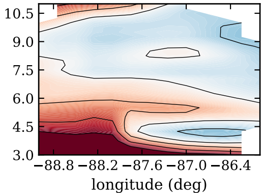
RF05, day 229, eflux (W/m 2 )
