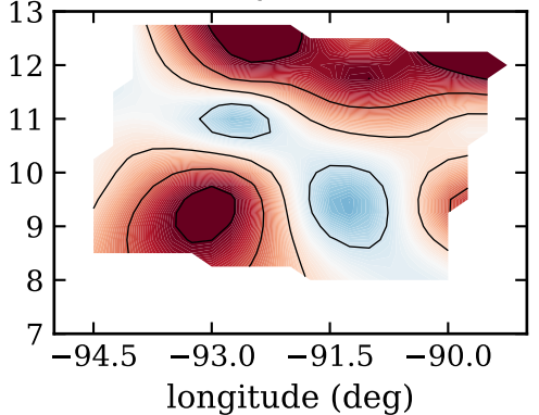
RF06, day 230, satfrac
