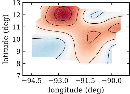
RF06, day 230, instab index (J/K/kg)
